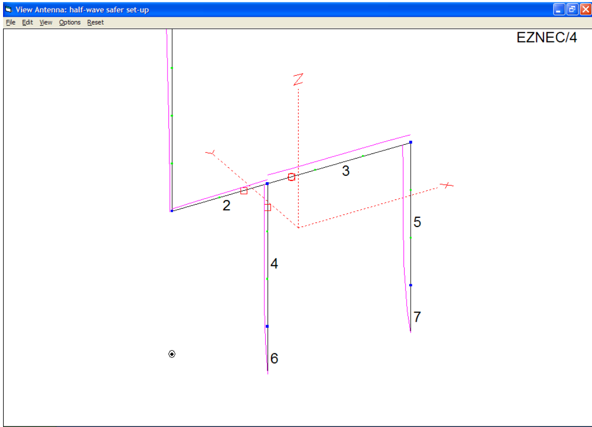
Figure 8 - Ground Wires added to Counterpoise (5 pF in wire 4, other loads are shorts)
