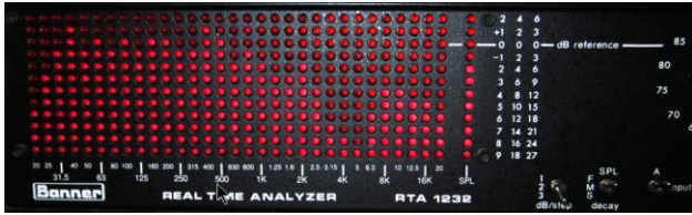
Fig 5: an L+R spectrum with a problem
